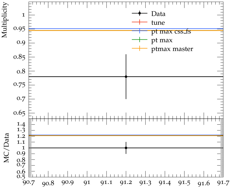
Mean K^*(892)^+ / K^*(892)^- multiplicity
