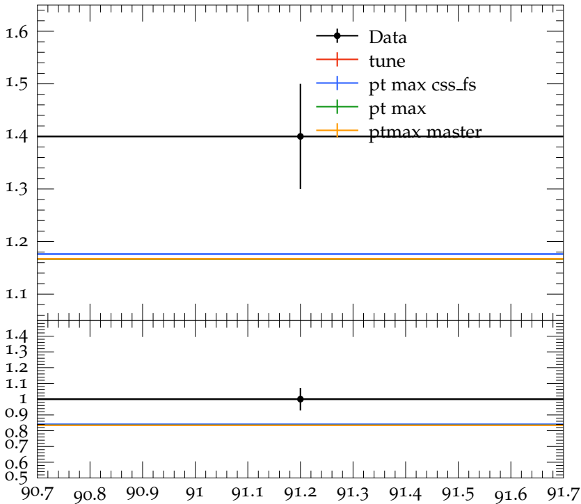
Mean \rho multiplicity
