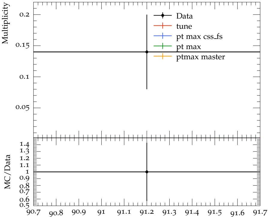
Mean f_0(980) multiplicity
