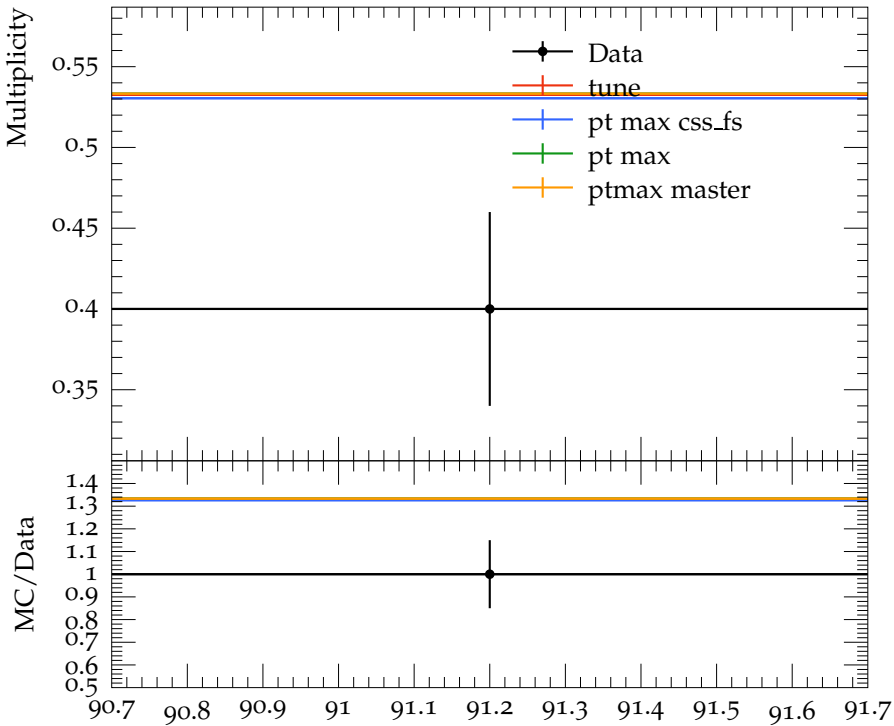
Mean D^0 multiplicity
