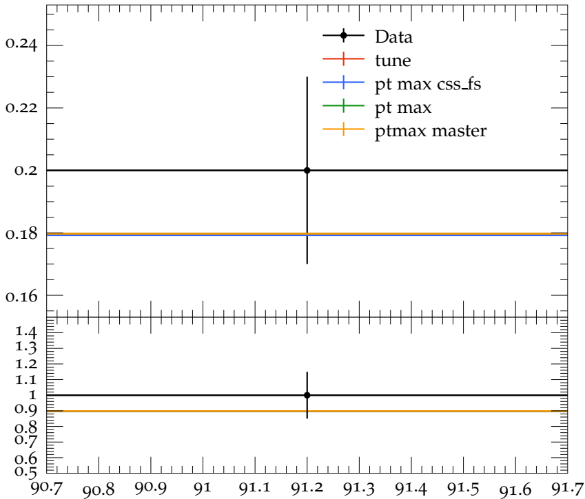
Mean D^+ multiplicity
