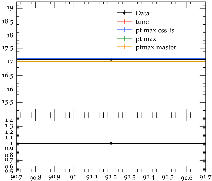
Mean \pi^+/\pi^- multiplicity
