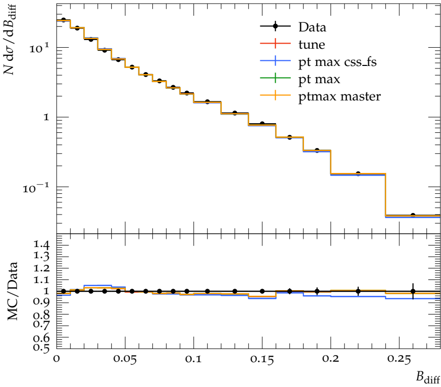
Difference in hemisphere broadening, B_{\text{diff}}
