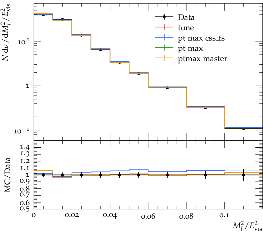
Light hemisphere masses, M_l^2/E_{\text{vis}}^2
