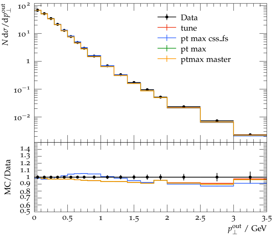
Out-of-plane p_{\perp} in GeV w.r.t. sphericity axes
