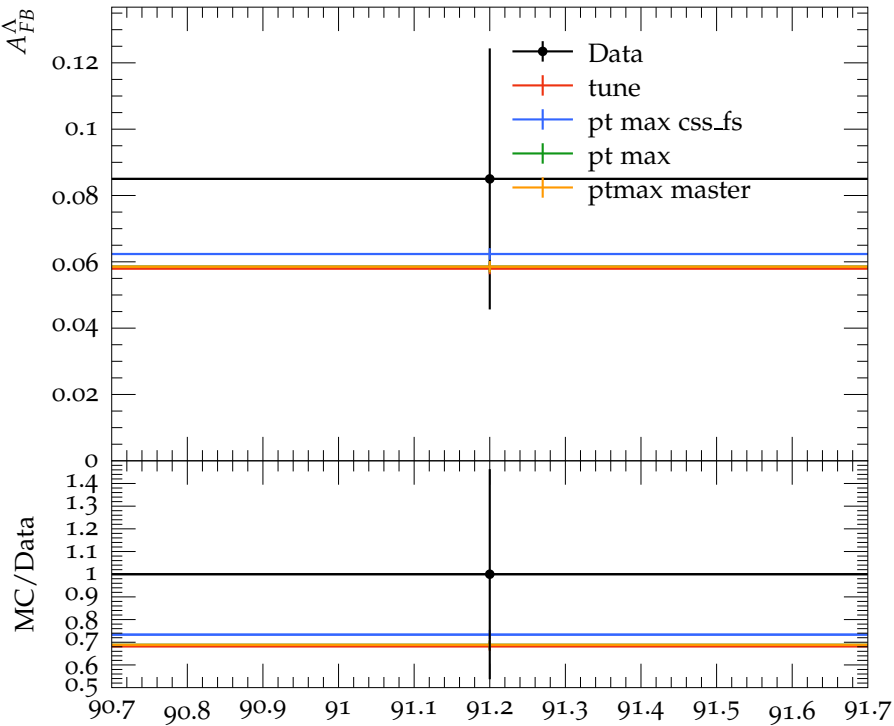
Forward-Backward asymmetry for \Lambda^0
