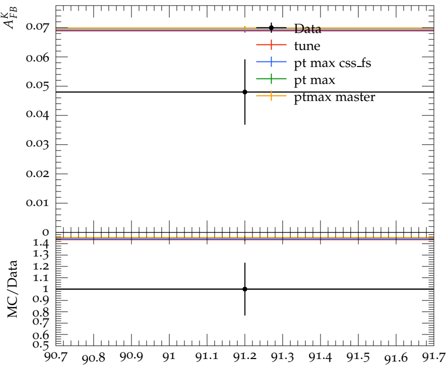
Forward-Backward asymmetry for K^\pm
