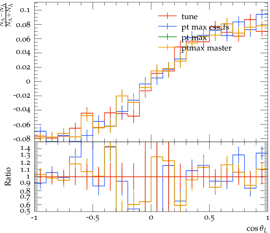
Asymmetry vs \cos \theta_L for \Lambda^0
