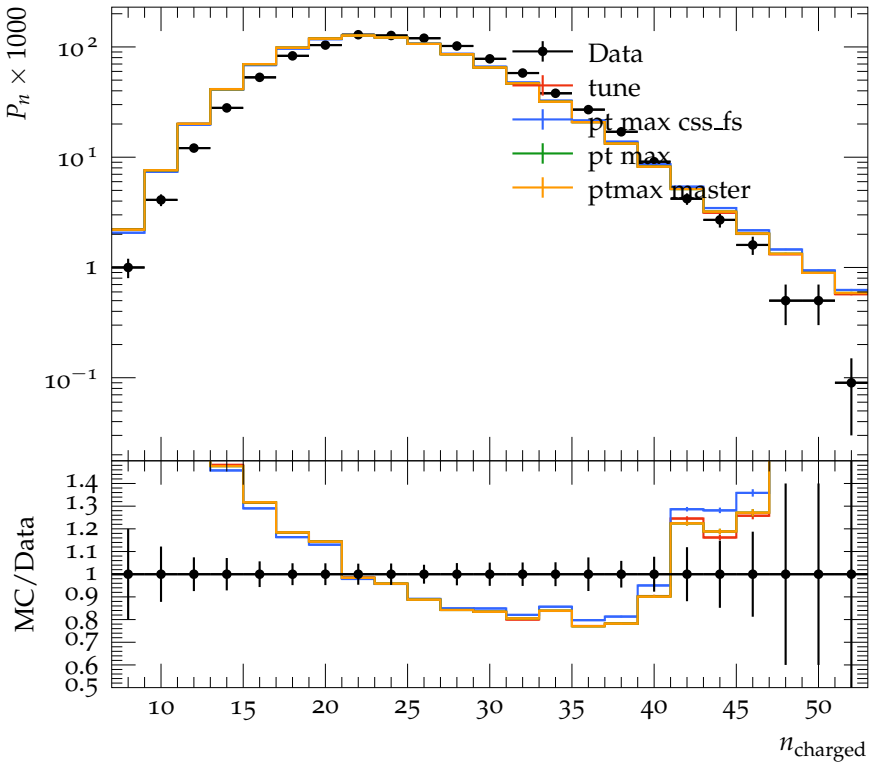
Charged pair particle multiplicity, 3-jets, y_{\text{cut}} = 0.04
