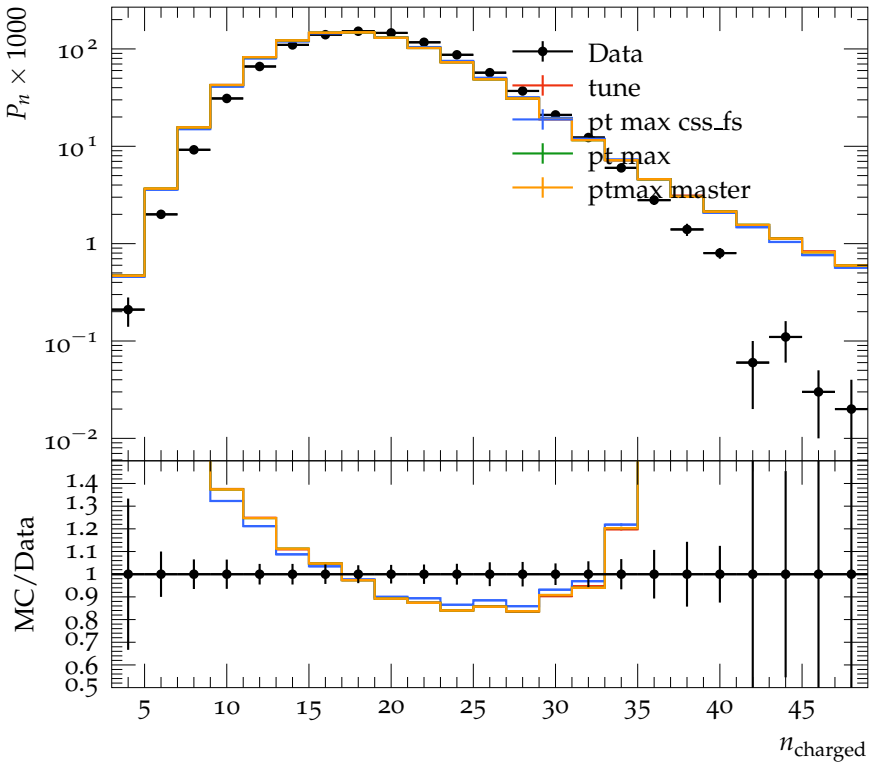
Charged pair particle multiplicity, 2-jets, y_{\text{cut}} = 0.04
