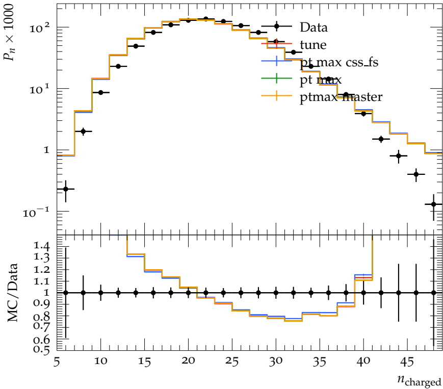
Charged pair particle multiplicity, 3-jets, y_{\text{cut}} = 0.02
