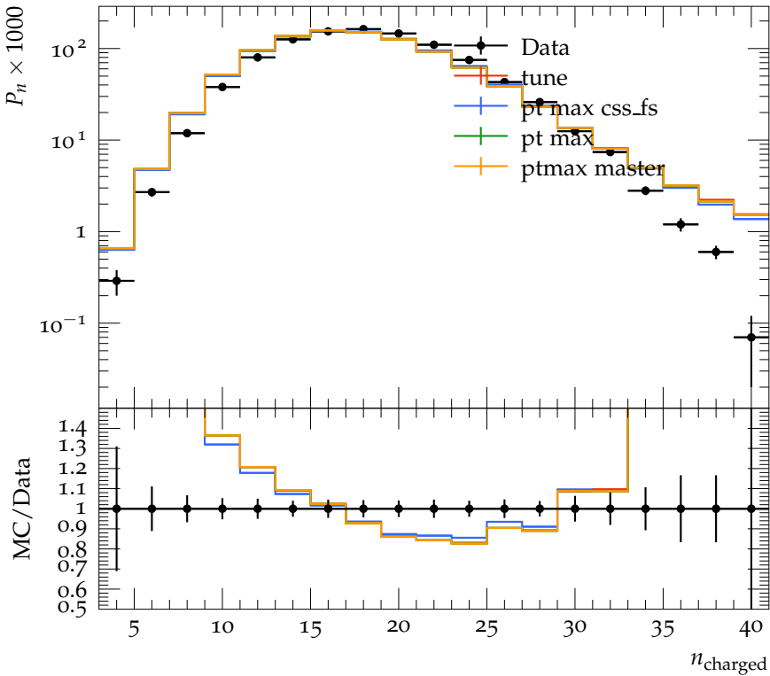
Charged pair particle multiplicity, 2-jets, y_{\text{cut}} = 0.02
