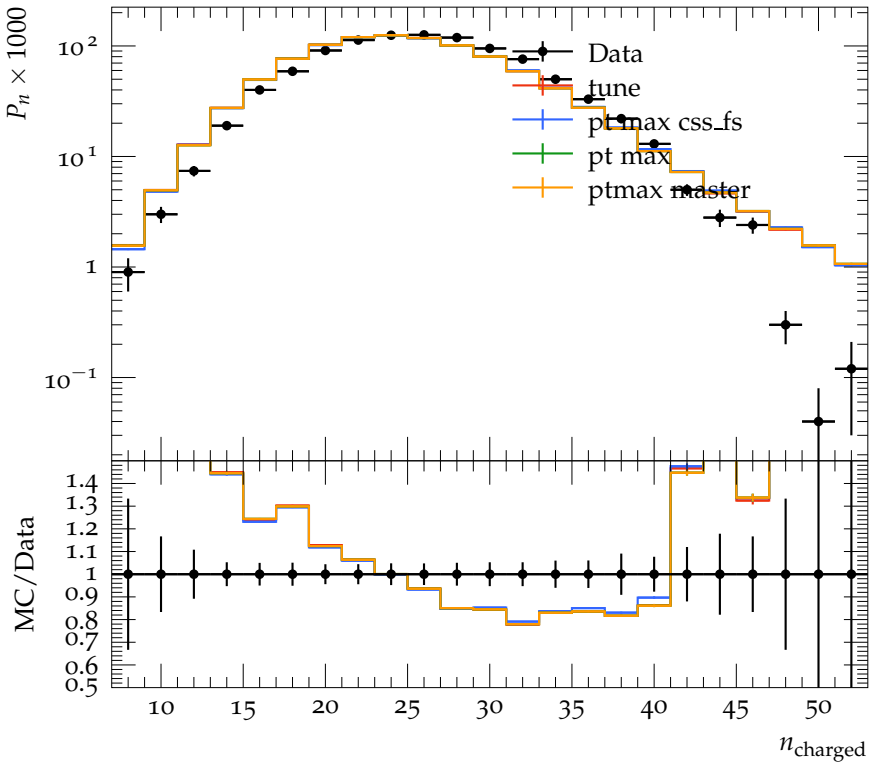
Charged pair particle multiplicity, 4-jets, y_{\text{cut}} = 0.01
