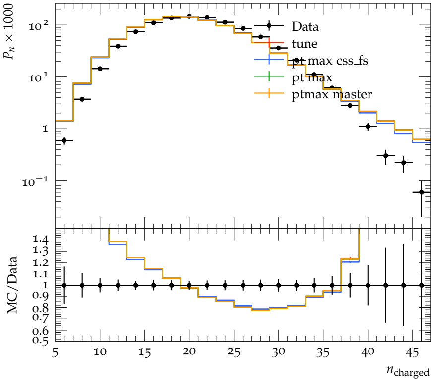
Charged pair particle multiplicity, 3-jets, y_{\text{cut}} = 0.01
