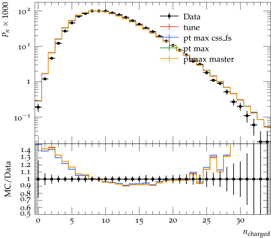
Charged Particle Multiplicity, single hemisphere
