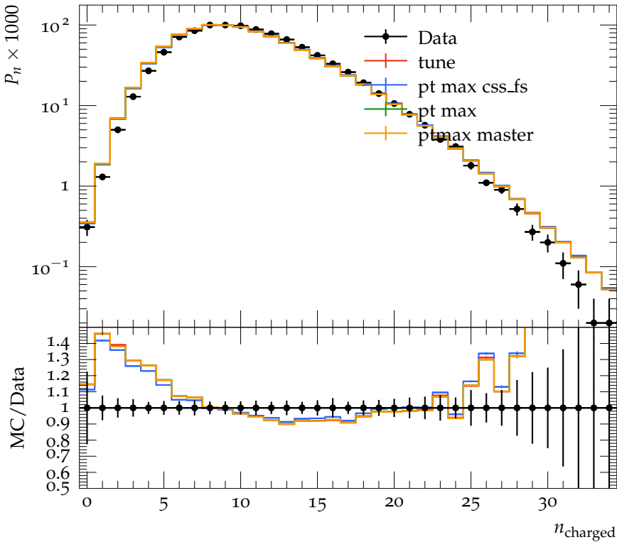
Charged Particle Multiplicity, single hemisphere, |y| < 5.0
