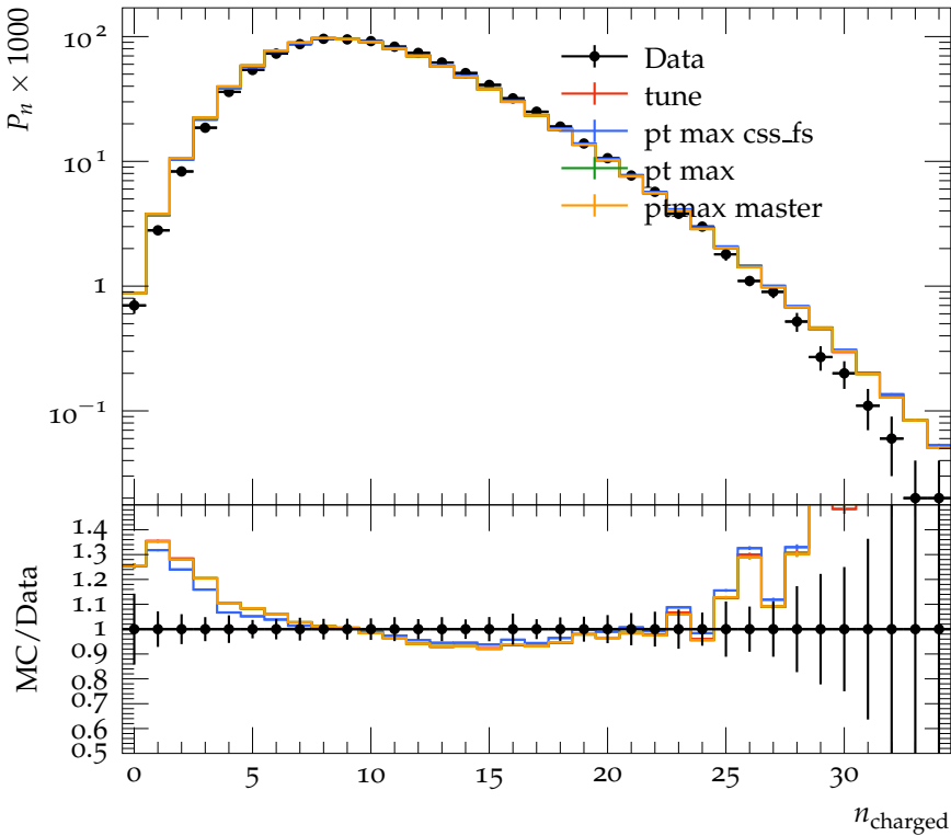
Charged Particle Multiplicity, single hemisphere, |y| < 4.0
