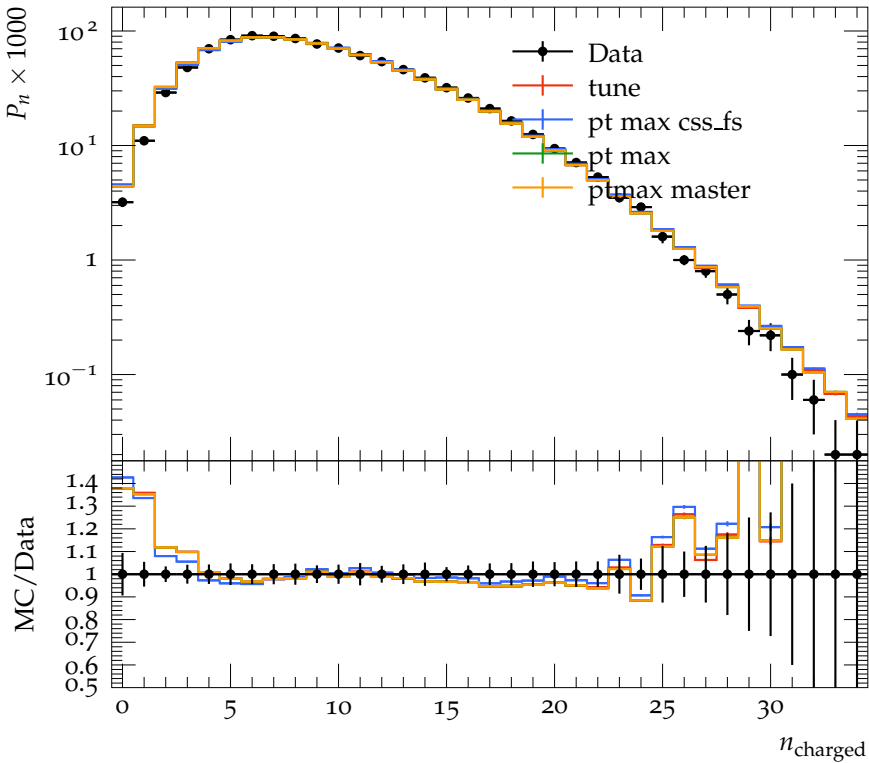
Charged Particle Multiplicity, single hemisphere, |y| < 3.0
