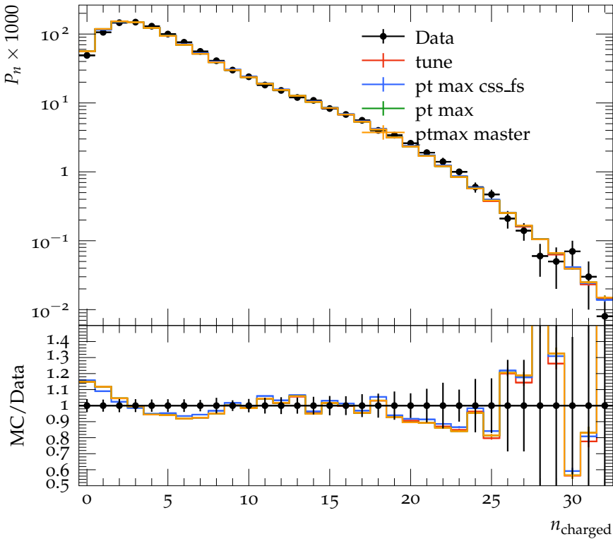
Charged Particle Multiplicity, single hemisphere, |y| < 1.5
