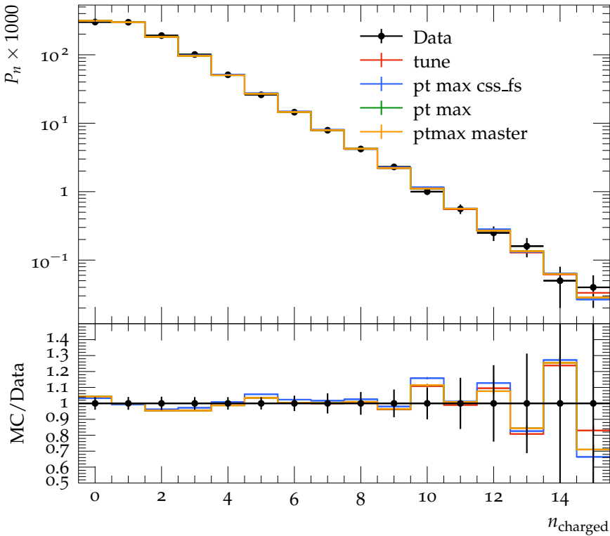
Charged Particle Multiplicity, single hemisphere, |y| < 0.5
