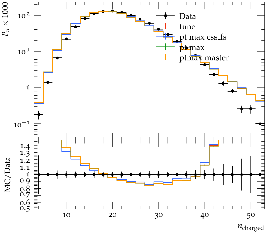
Charged Particle Multiplicity, both hemispheres
