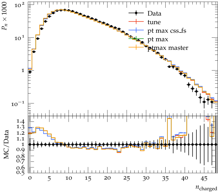
Charged Particle Multiplicity, both hemispheres, |y| < 2.0
