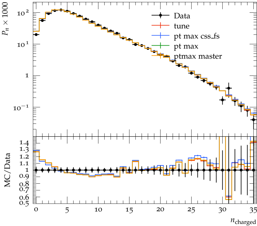
Charged Particle Multiplicity, both hemispheres, |y| < 1.0
