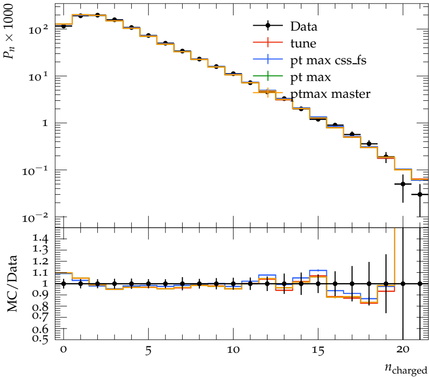
Charged Particle Multiplicity, both hemispheres, |y| < 0.5
