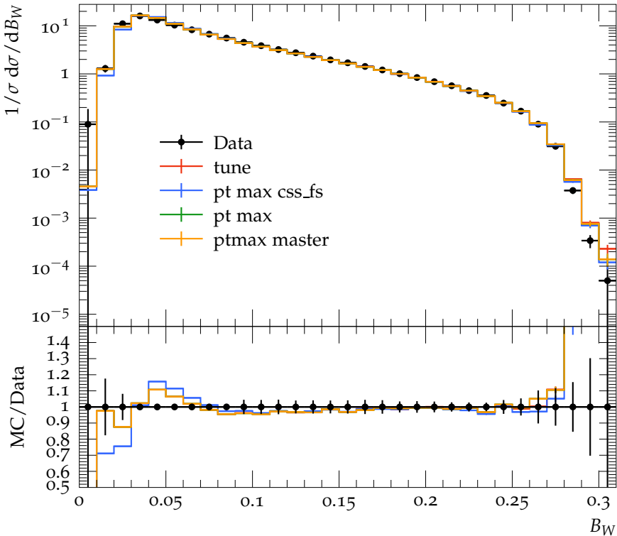
Wide jet broadening ( E_{\text{CMS}} = 91.2 \text{ GeV} )
