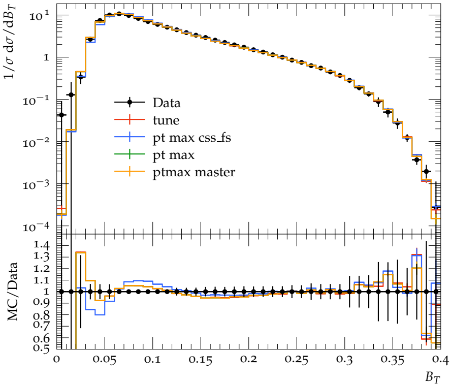
Total jet broadening ( E_{\text{CMS}} = 91.2 \text{ GeV} )
