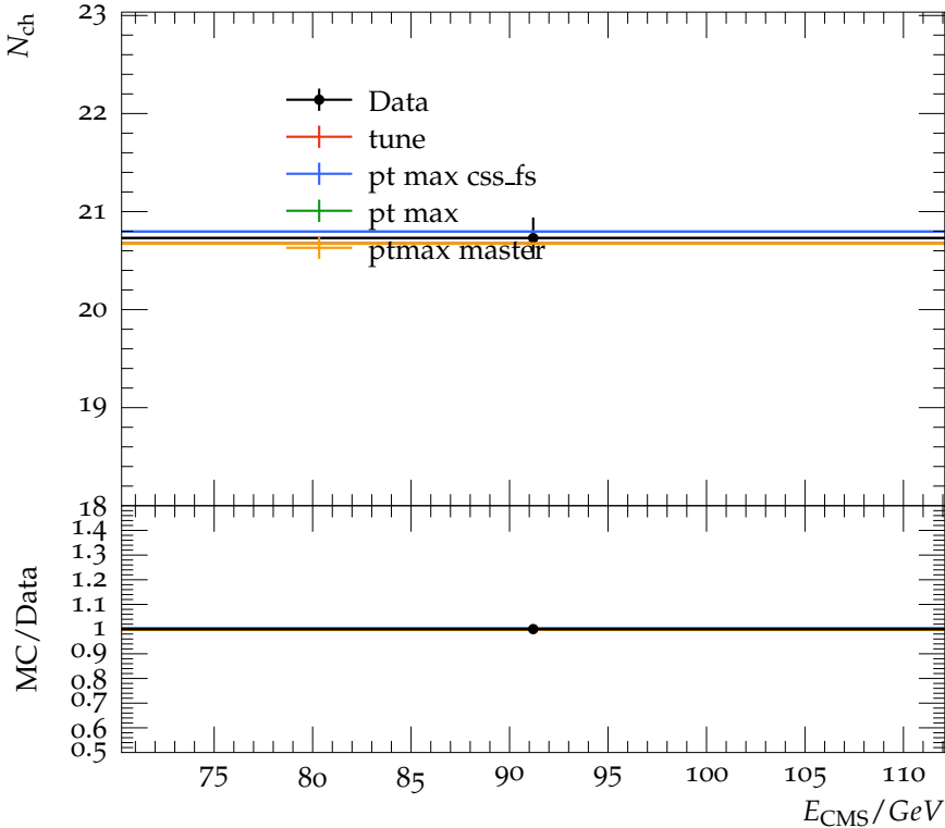
Charged multiplicity at a function of energy
