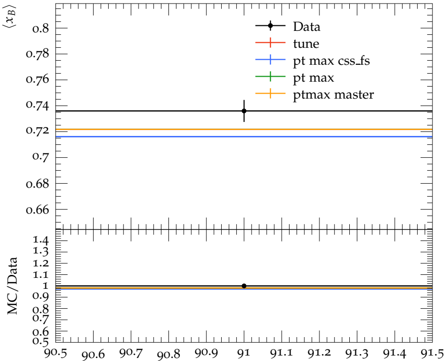
Mean of b quark fragmentation function f(x_B^{\text{lead}})
