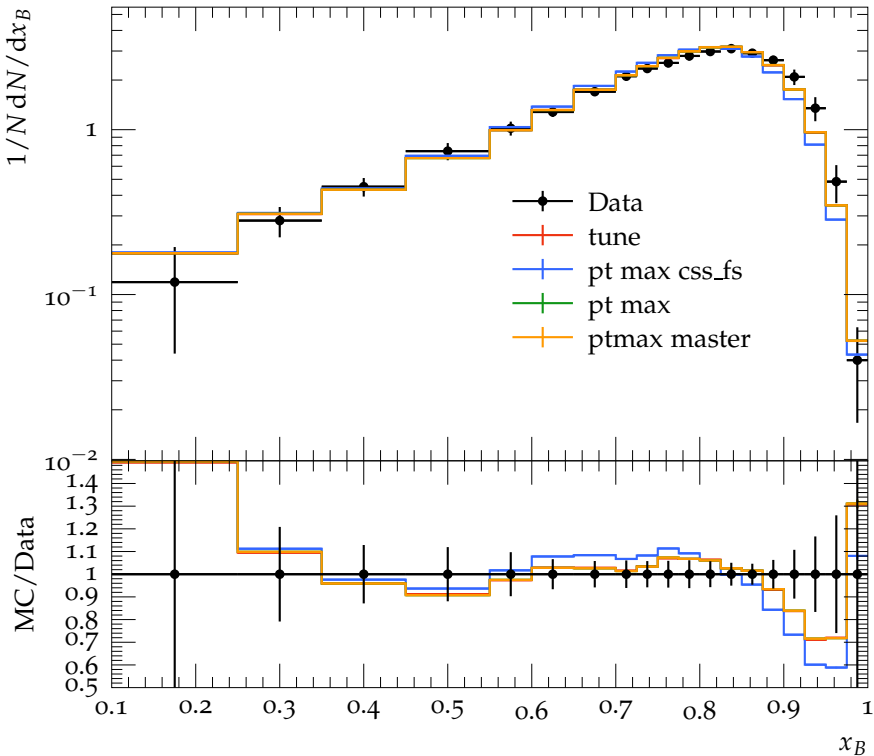
b quark fragmentation function f(x_B^{\text{weak}})
