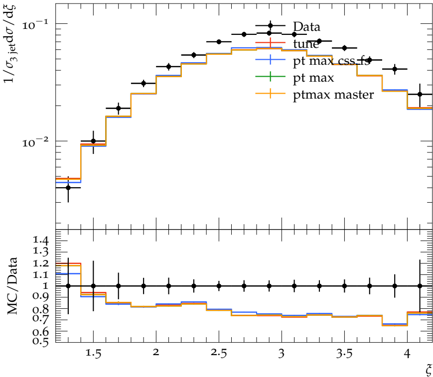
Log Scaled momentum fraction for \Lambda^0 in 3rd jet (3-jet events)
