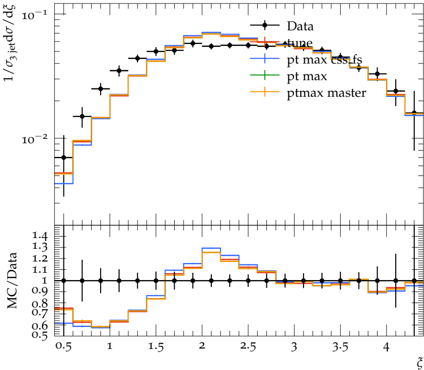
Log Scaled momentum fraction for \Lambda^0 in 1st jet (3-jet events)
