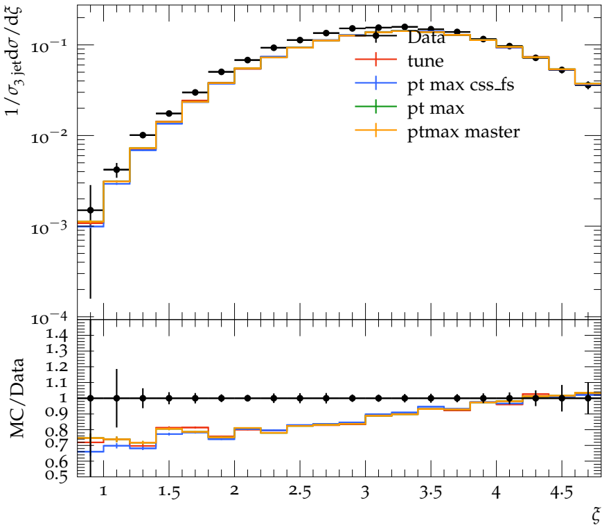
Log Scaled momentum fraction for K_S^0 in 3rd jet (3-jet events)
