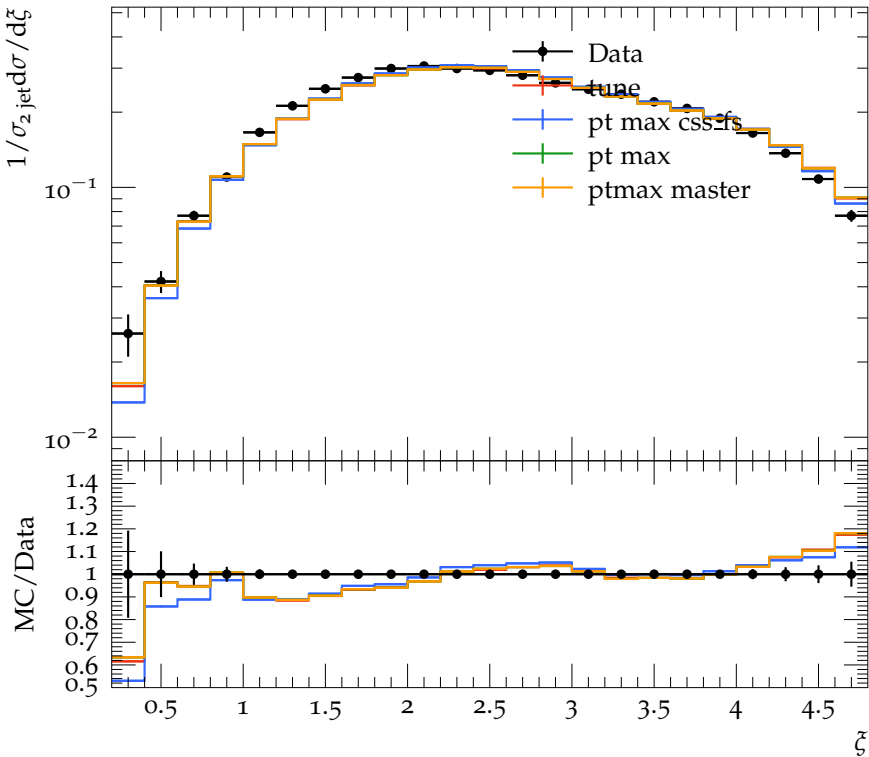
Log Scaled momentum fraction for K_S^0 (2-jet events)
