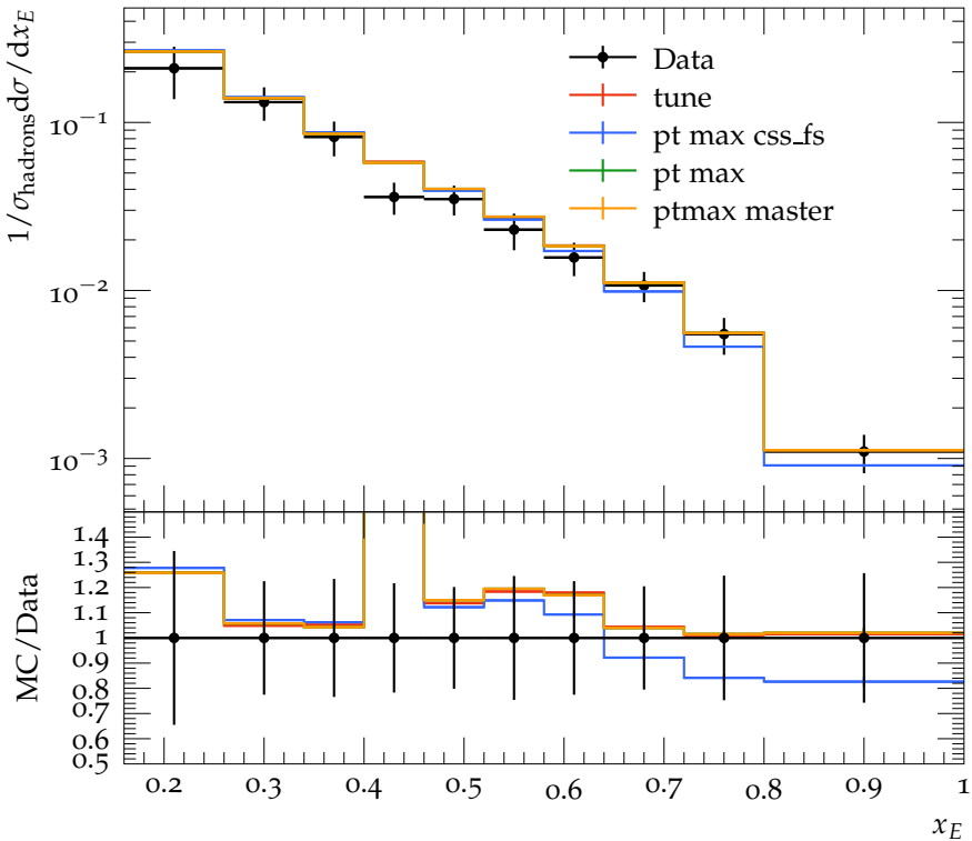
Scaled energy fraction for \eta' (all events)
