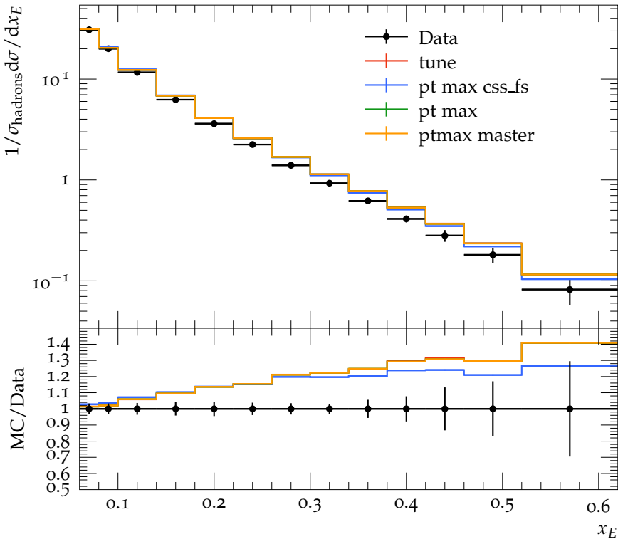
Scaled energy fraction for \pi^0 (all events)
