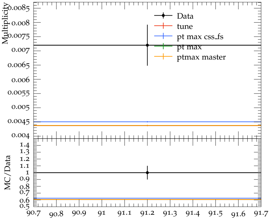
Mean \Xi(1530) multiplicity
