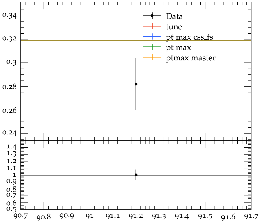
Mean \eta multiplicity
