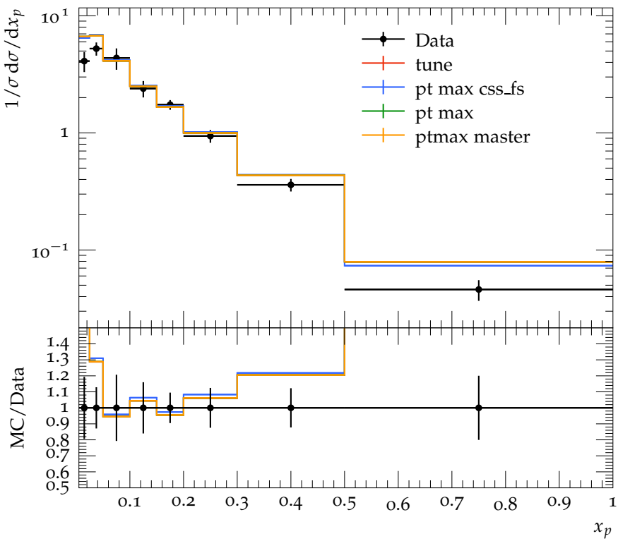
K^{*0}(892) spectrum
