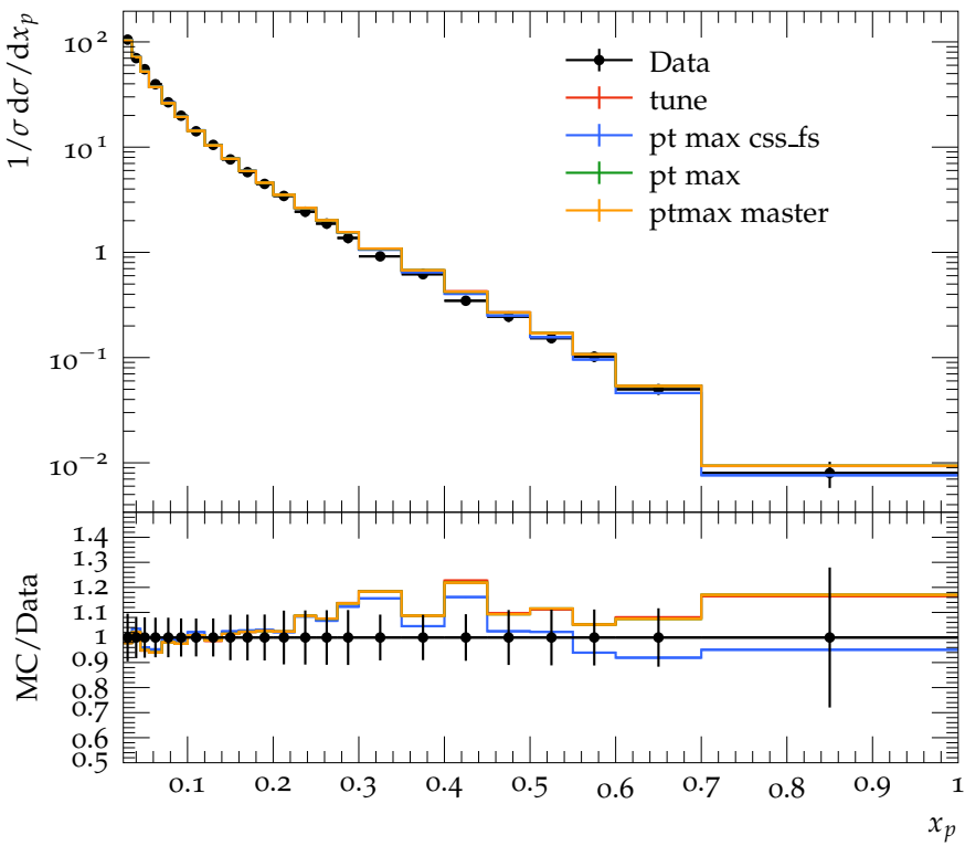
\pi^0 spectrum
