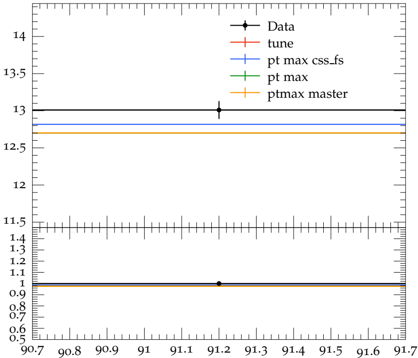
Mean charged multiplicity for rapidity |Y| < 2.0
