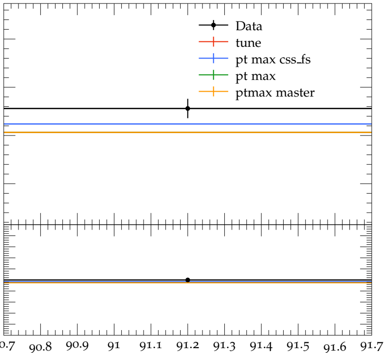
Mean charged multiplicity for rapidity |Y| < 1.5
