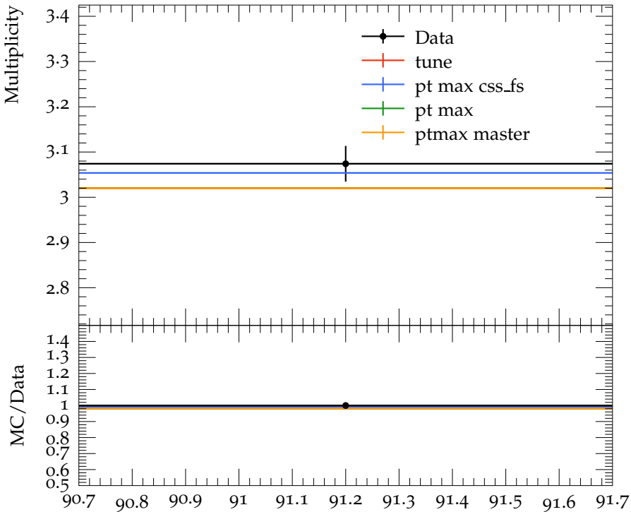
Mean charged multiplicity for rapidity |Y| < 0.5
