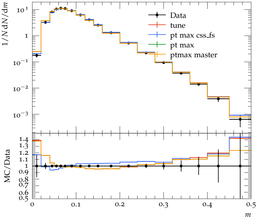
Thrust minor, m (charged)
