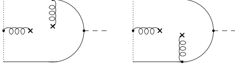
Figure 4.5: Diagrams contributing to the gluon condensate \langle \frac{\alpha_s}{\pi} G^2 \rangle .
