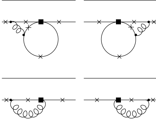
Figure 6.2: Penguin contractions of Q_{1,...,6} (top line) and the chromomagnetic dipole operator Q_8 (bottom line) contributing to the hard-vertex corrections of T_i^I at \mathcal{O}(\alpha_s) . Crosses denote possible photon emission vertices.
