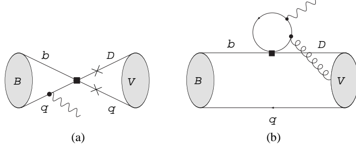
Figure 7.1: (a) Weak annihilation diagram where photon emission from the B meson spectator quark is power-suppressed. The crosses denote possible photon emission vertices for Q_{5,6} only. (b) soft-gluon emission from a quark loop, where there is also a second diagram in which the gluon is picked up by the B meson.
