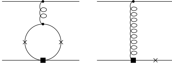
Figure 6.3: Penguin contractions of Q_{1,...,6} (left) and the chromomagnetic dipole operator Q_{8g} (right) contributing to the hard-scattering kernel T_i^{II} at \mathcal{O}(\alpha_s) . Crosses denote possible photon emission vertices at leading order. Photon emission from the other quark lines power-suppressed. Photon emission from the final state meson for Q_{8g} breaks factorisation.
