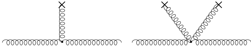
Figure 3.3: The interactions of the background field \mathcal{A}_\mu^a (denoted by a cross) with the quantum field a_\mu^a corresponding to \mathcal{L}_{int}^{Aaa} and \mathcal{L}_{int}^{AAaa} respectively.
