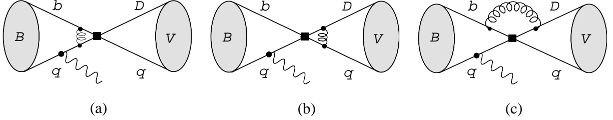
Figure 7.2: Example radiative corrections to weak annihilation. The corrections to the B vertex in (a) are known [71, 178] and those to the V vertex in (b) are included in f_V . For the non-factorisable corrections in (c) only preliminary results are available [177].
