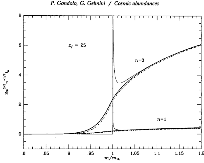
Figure 2.2 Relativistic thermal average near a threshold (thick solid line) compared to the result from the expansion in powers of x^{-1} (thin line). Figure from Ref. [17].
