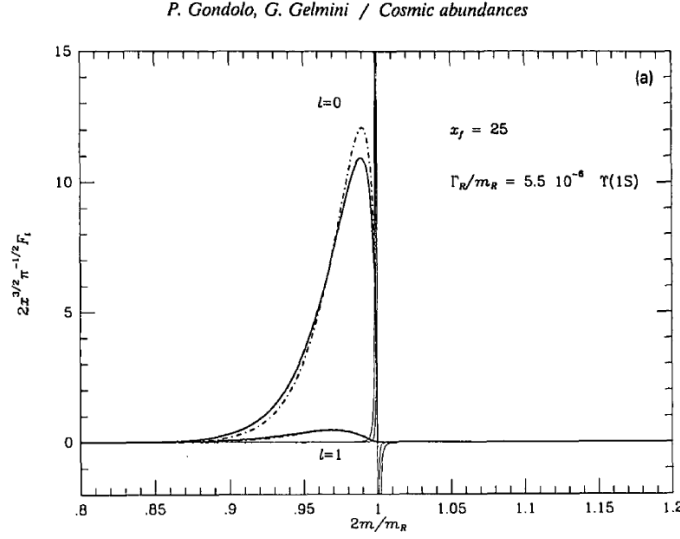
Figure 2.3 Relativistic thermal average in a resonance (thick solid line) compared to the result from the expansion in powers of x^{-1} (thin line). Figure from Ref. [17].
