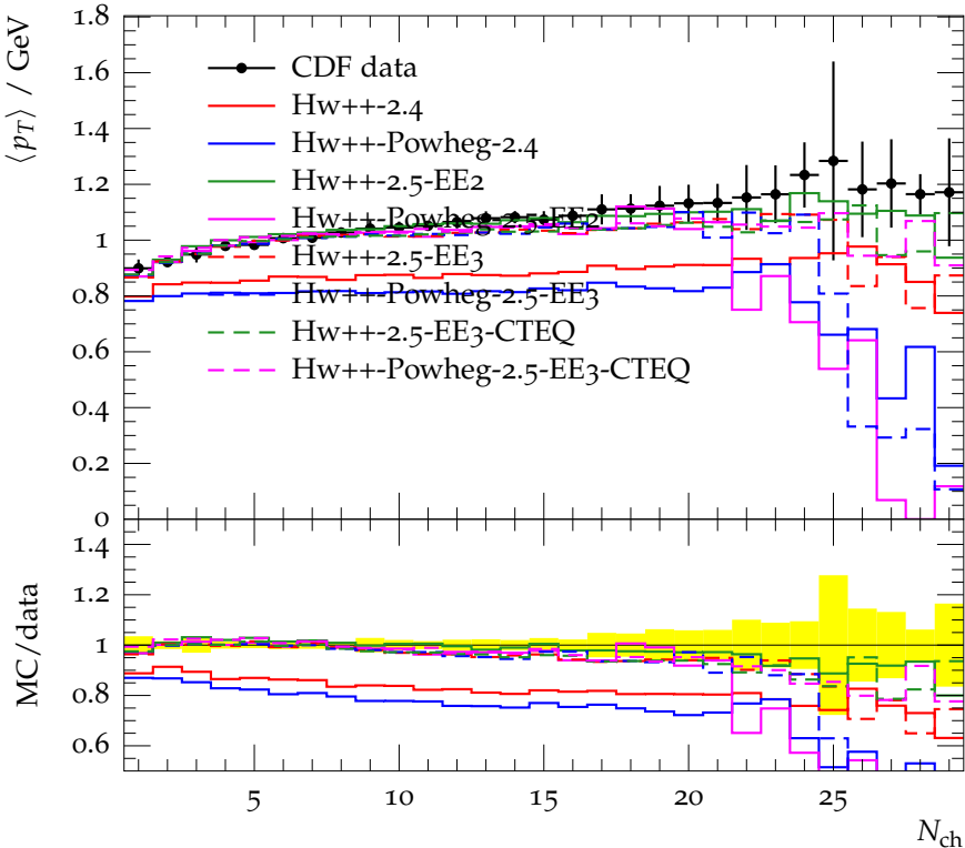
Average charged p_{\perp} vs charged multiplicity, p_{\perp}(Z) < 10 GeV
